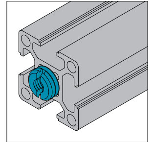
Hole Reducer Bolt M12/M6 PG30 with core hole-Φ10(M12)
