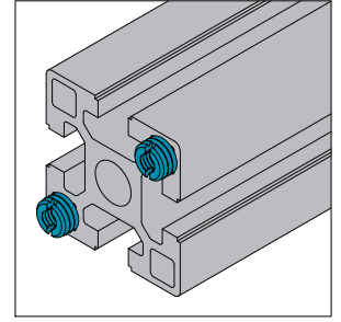
Hole Reducer Bolt M10/M6 PG45 with square corner hole-8x8(M10)
