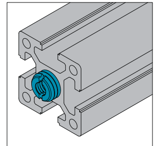
Hole Reducer Bolt M14/M8 PG40/PG45/PG50/PG60 with core hole-Φ12(M14)
