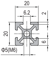
PG20 20x20 4 slots
