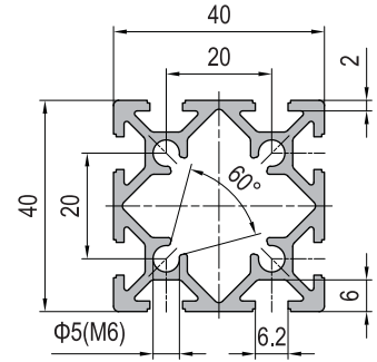
PG20 40x40 8 slots
