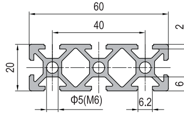
PG20 20x60 8 slots
