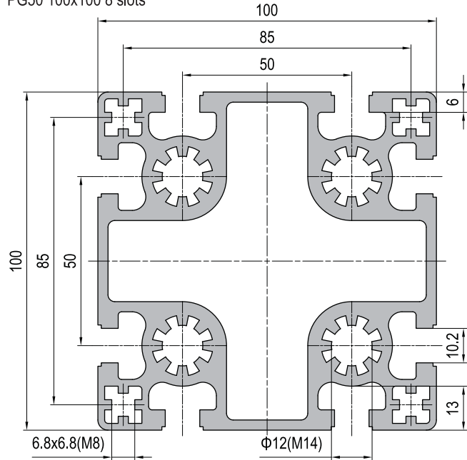
PG50 100x100 8 slots
